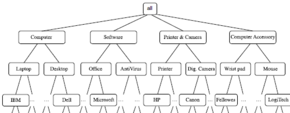
A concept hierarchy for AllElectronics computer items.
